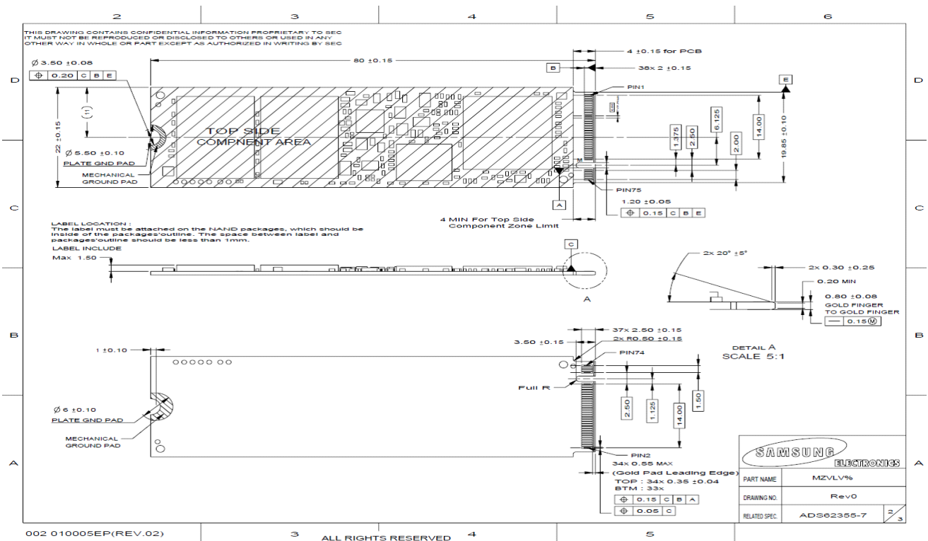
[Figure 1] M.2 Package
